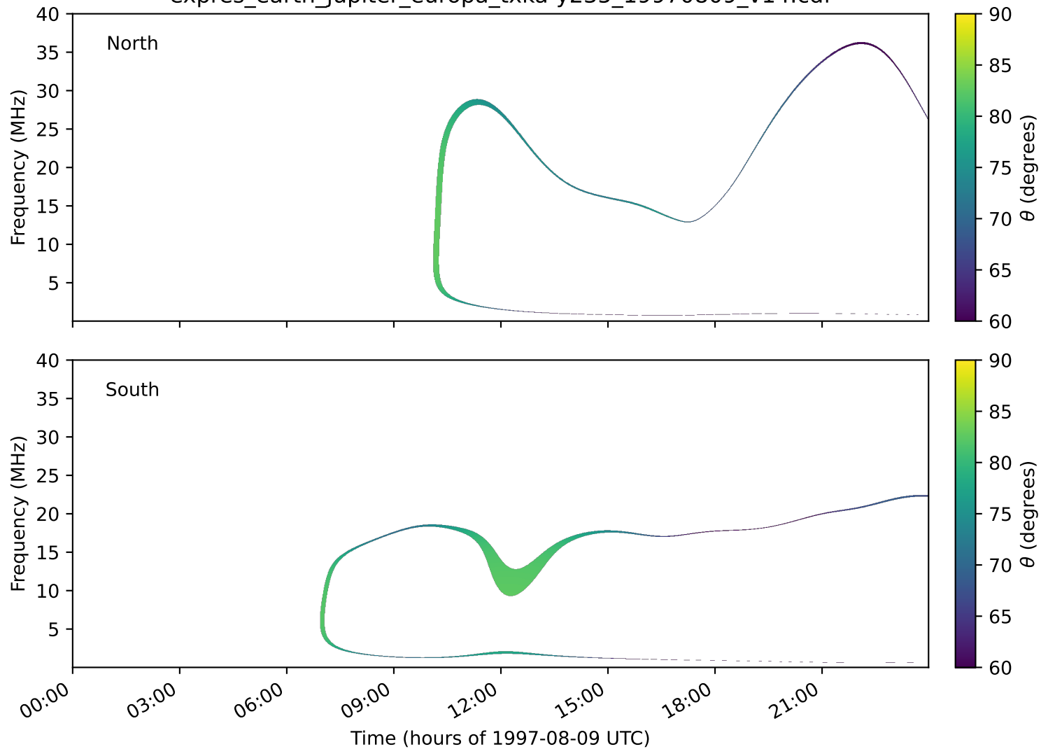
expres_earth_jupiter_europa_txka-y235_19970809_v14.cdf
