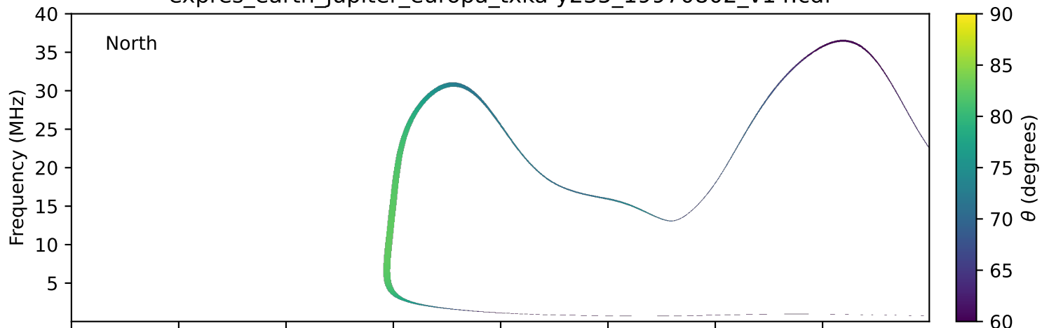
expres_earth_jupiter_europa_txka-y235_19970802_v14.cdf
