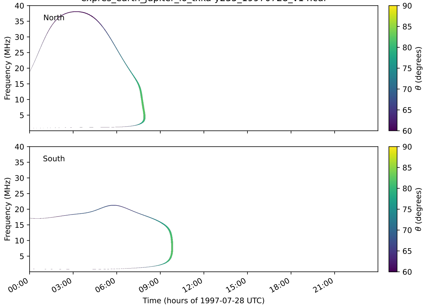
expres_earth_jupiter_io_txka-y235_19970728_v14.cdf
