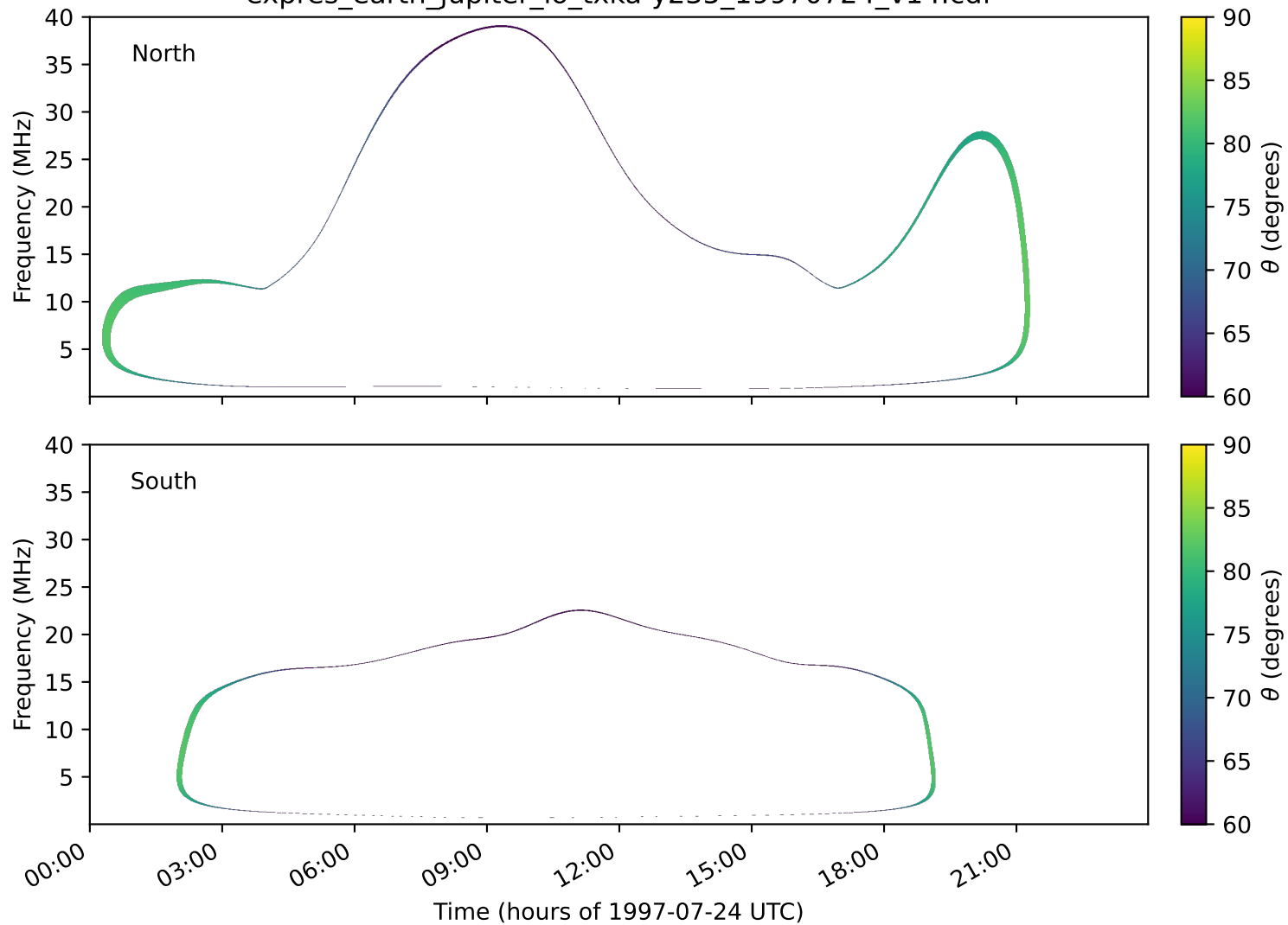
expres_earth_jupiter_io_txka-y235_19970724_v14.cdf
