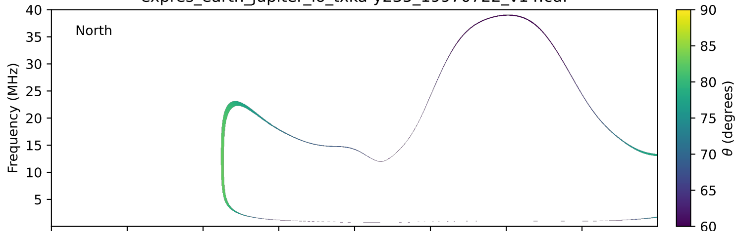
expres_earth_jupiter_io_txka-y235_19970722_v14.cdf
