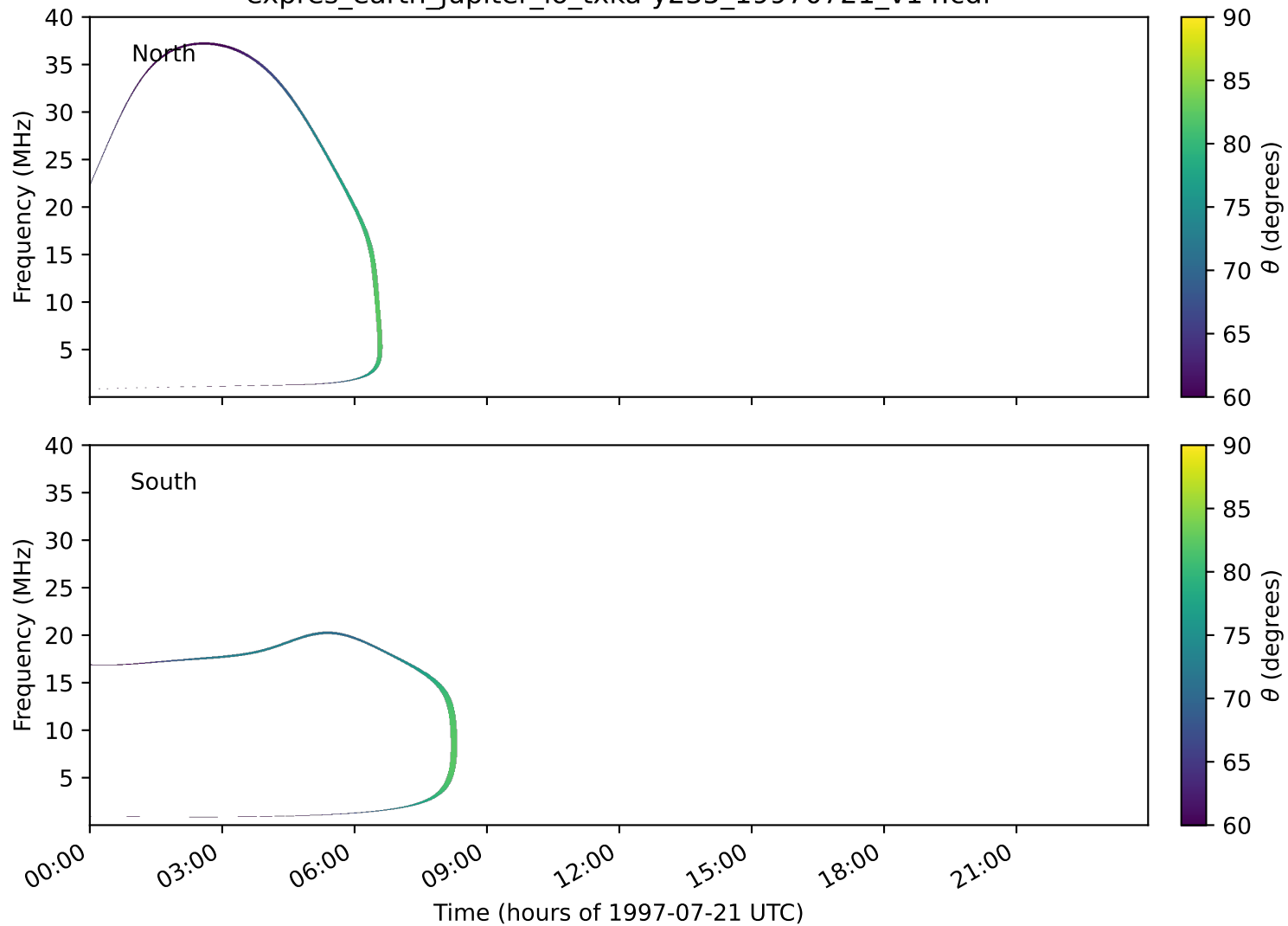
expres_earth_jupiter_io_txka-y235_19970721_v14.cdf
