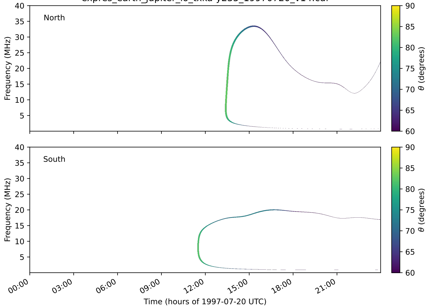
expres_earth_jupiter_io_txka-y235_19970720_v14.cdf
