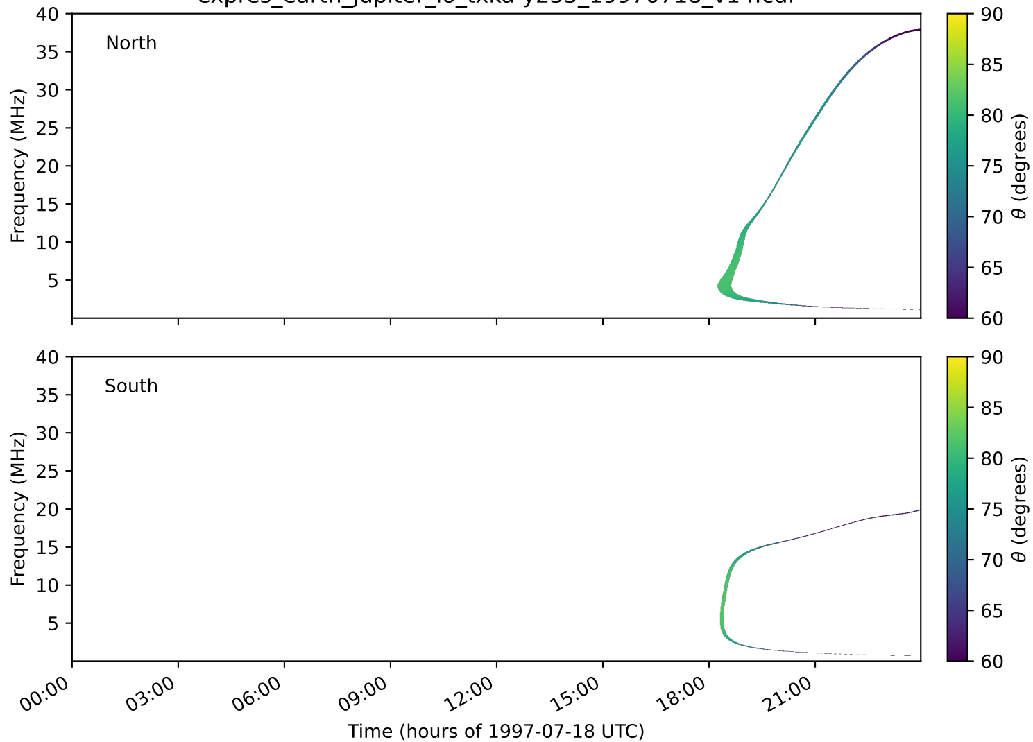
expres_earth_jupiter_io_txka-y235_19970718_v14.cdf
