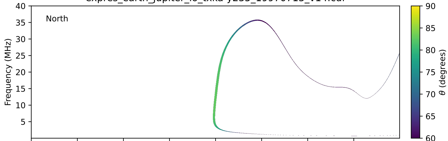
expres_earth_jupiter_io_txka-y235_19970713_v14.cdf
