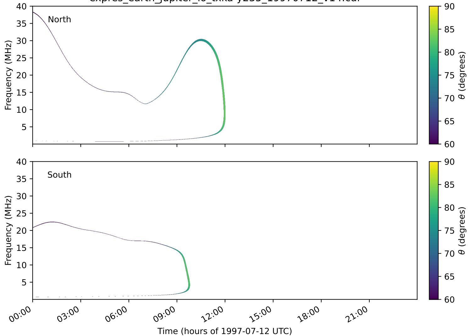
expres_earth_jupiter_io_txka-y235_19970712_v14.cdf
