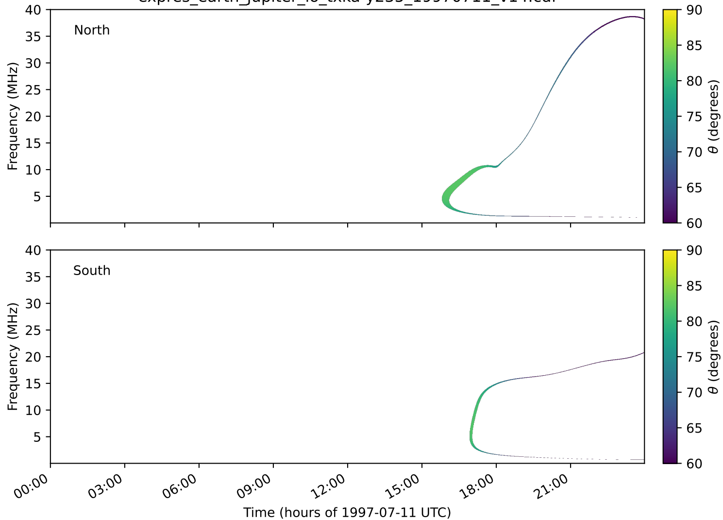
expres_earth_jupiter_io_txka-y235_19970711_v14.cdf
