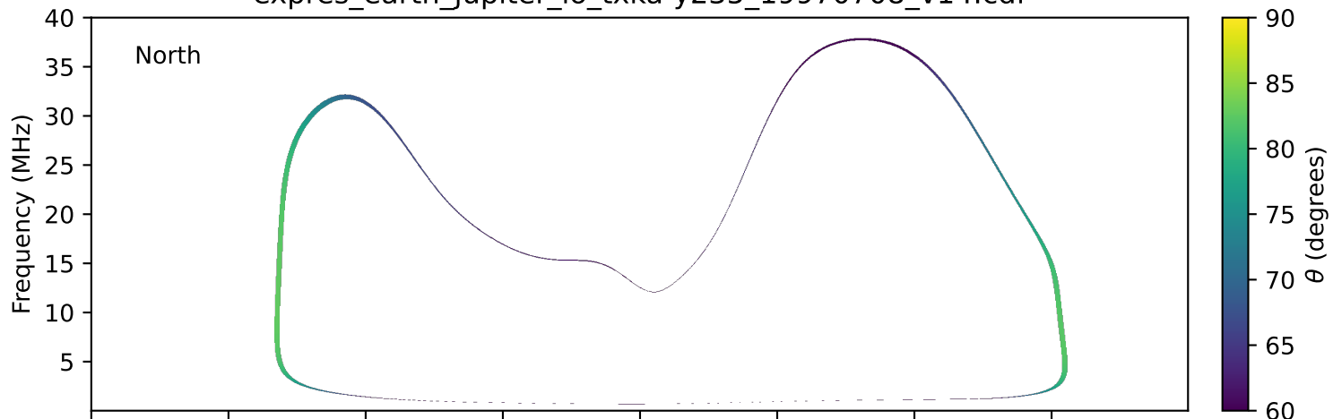
expres_earth_jupiter_io_txka-y235_19970708_v14.cdf
