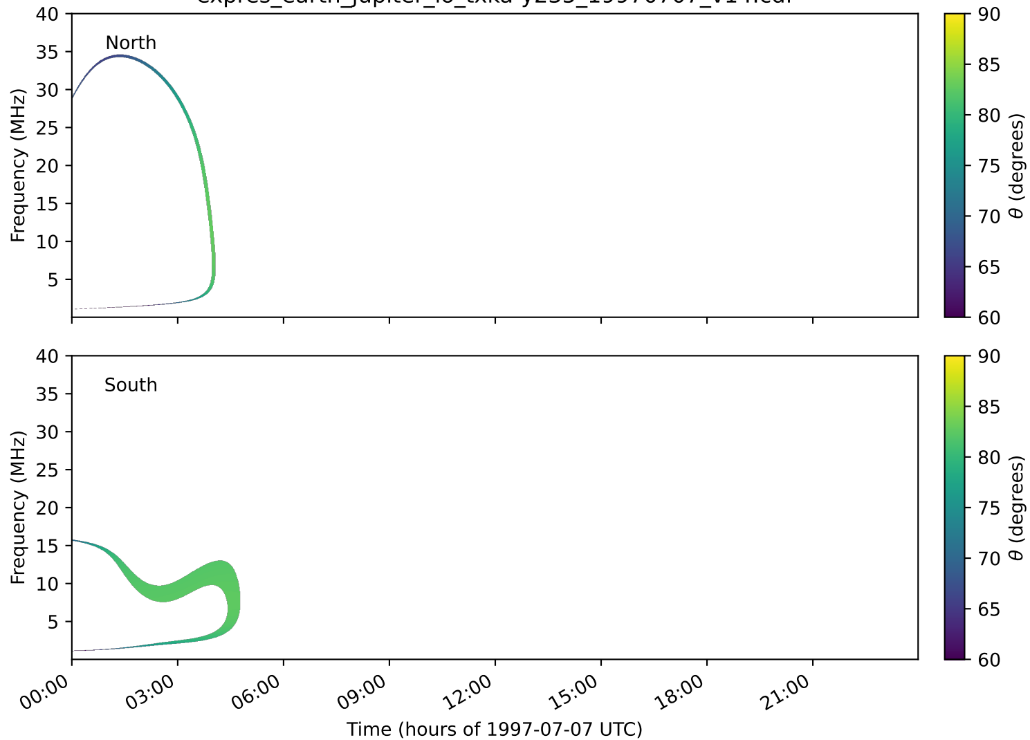
expres_earth_jupiter_io_txka-y235_19970707_v14.cdf
