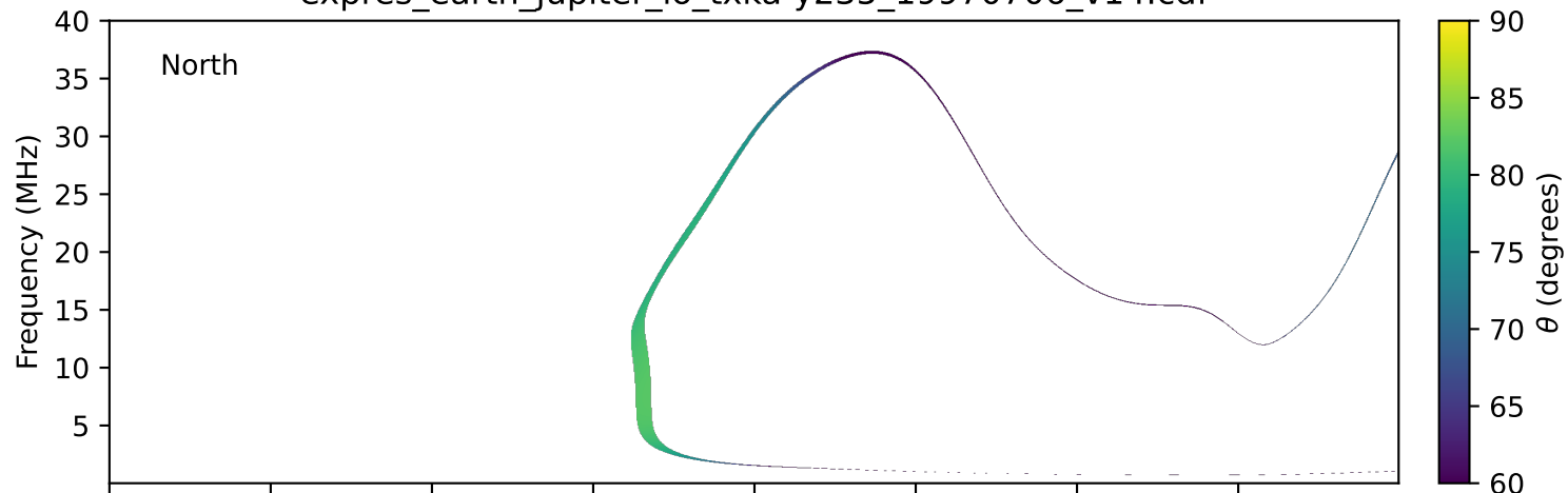
expres_earth_jupiter_io_txka-y235_19970706_v14.cdf
