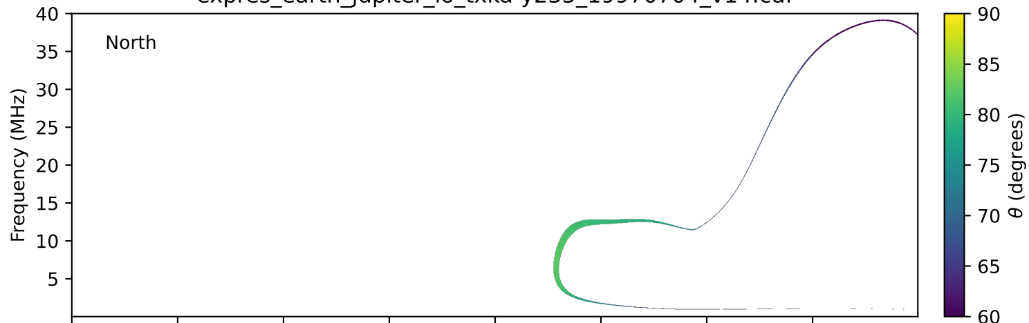
expres_earth_jupiter_io_txka-y235_19970704_v14.cdf
