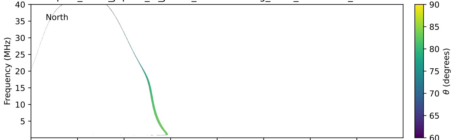
expres_earth_jupiter_io_jrm33_lossc-wid1deg_3kev_19970728_v11.cdf
