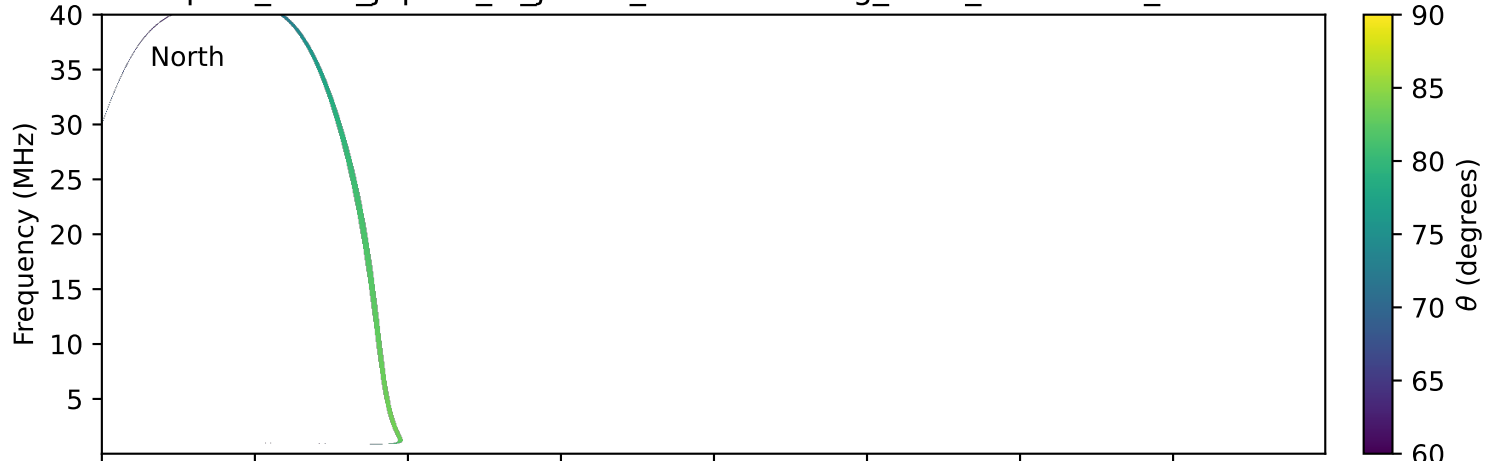
expres_earth_jupiter_io_jrm33_lossc-wid1deg_3kev_19970714_v11.cdf
