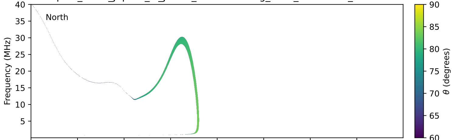
expres_earth_jupiter_io_jrm33_lossc-wid1deg_3kev_19970705_v11.cdf
