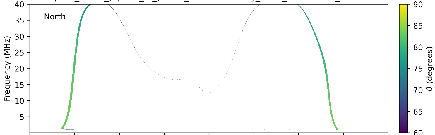
expres_earth_jupiter_io_jrm33_lossc-wid1deg_3kev_19970701_v11.cdf
