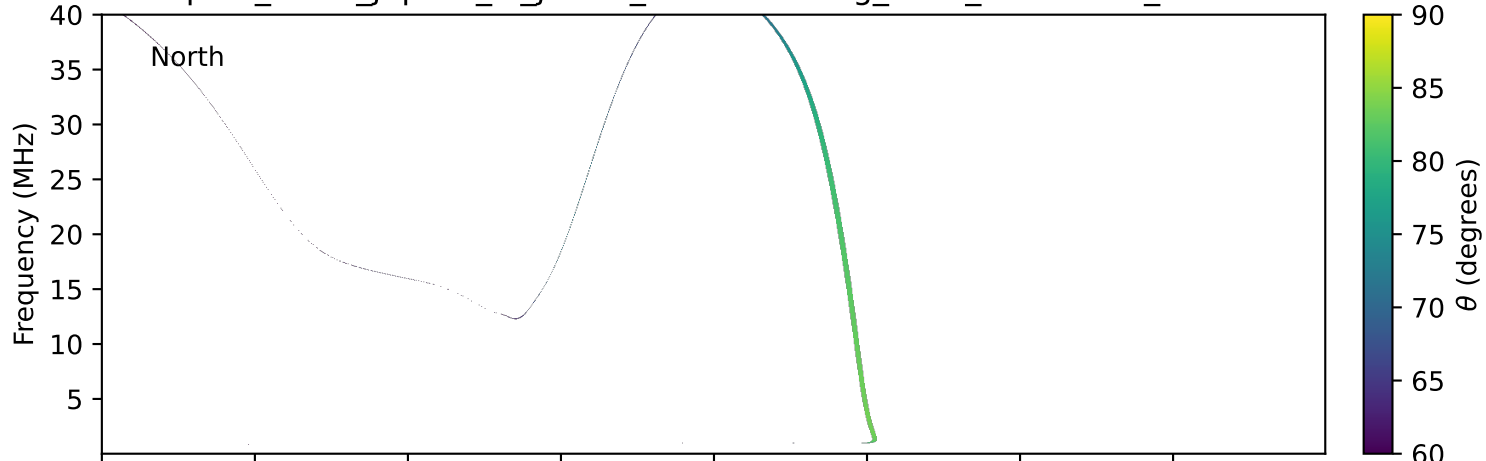
expres_earth_jupiter_io_jrm09_lossc-wid1deg_3kev_19970726_v11.cdf
