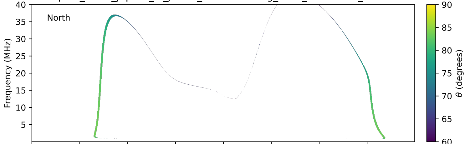
expres_earth_jupiter_io_jrm09_lossc-wid1deg_3kev_19970708_v11.cdf
