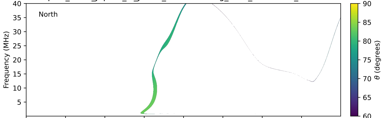
expres_earth_jupiter_io_jrm09_lossc-wid1deg_3kev_19970706_v11.cdf
