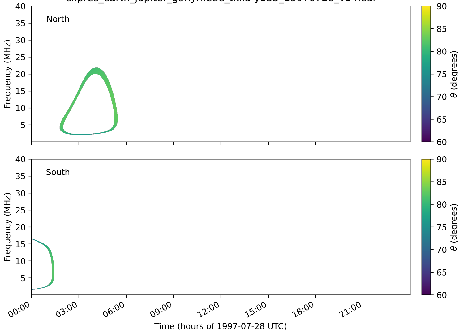
expres_earth_jupiter_ganymede_txka-y235_19970728_v14.cdf
