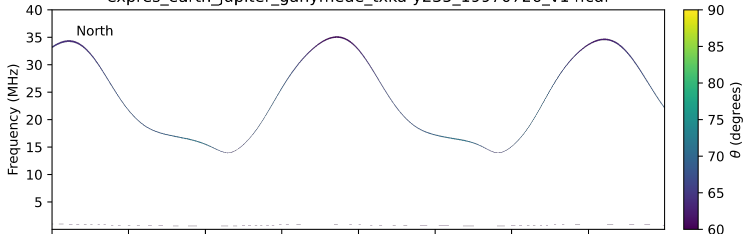
expres_earth_jupiter_ganymede_txka-y235_19970726_v14.cdf
