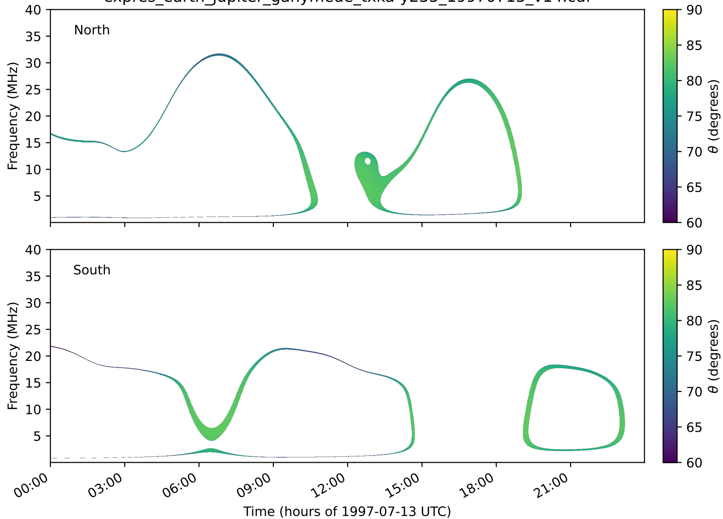
expres_earth_jupiter_ganymede_txka-y235_19970713_v14.cdf
