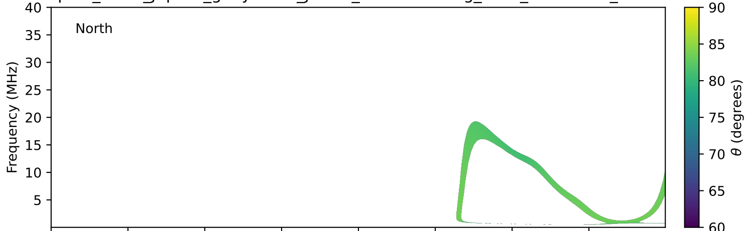
expres_earth_jupiter_ganymede_jrm33_lossc-wid1deg_3kev_19970703_v11.cdf
