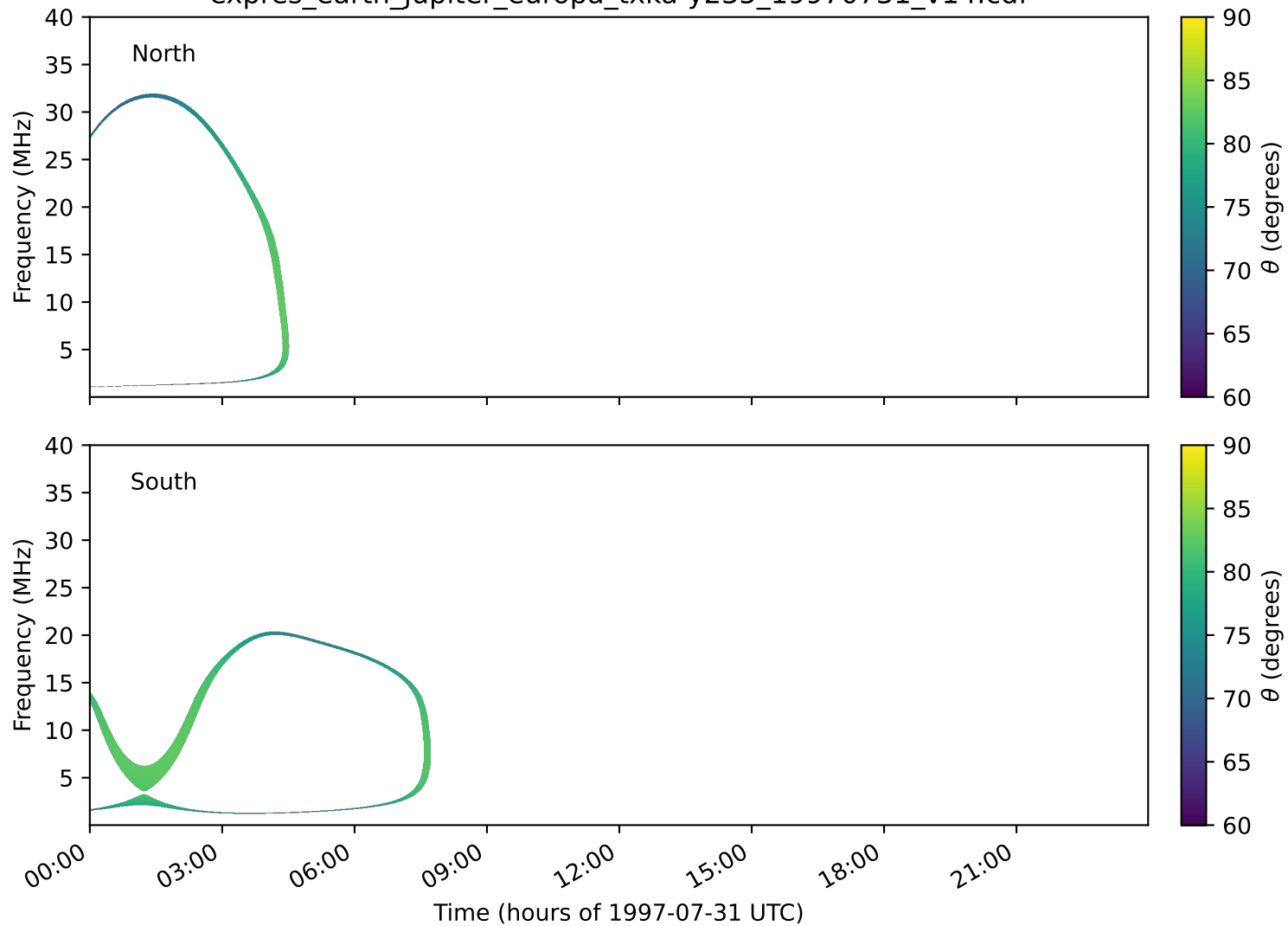
expres_earth_jupiter_europa_txka-y235_19970731_v14.cdf
