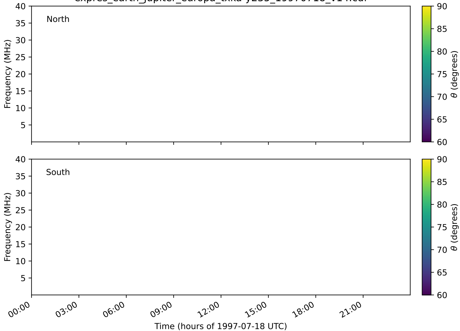
expres_earth_jupiter_europa_txka-y235_19970718_v14.cdf
