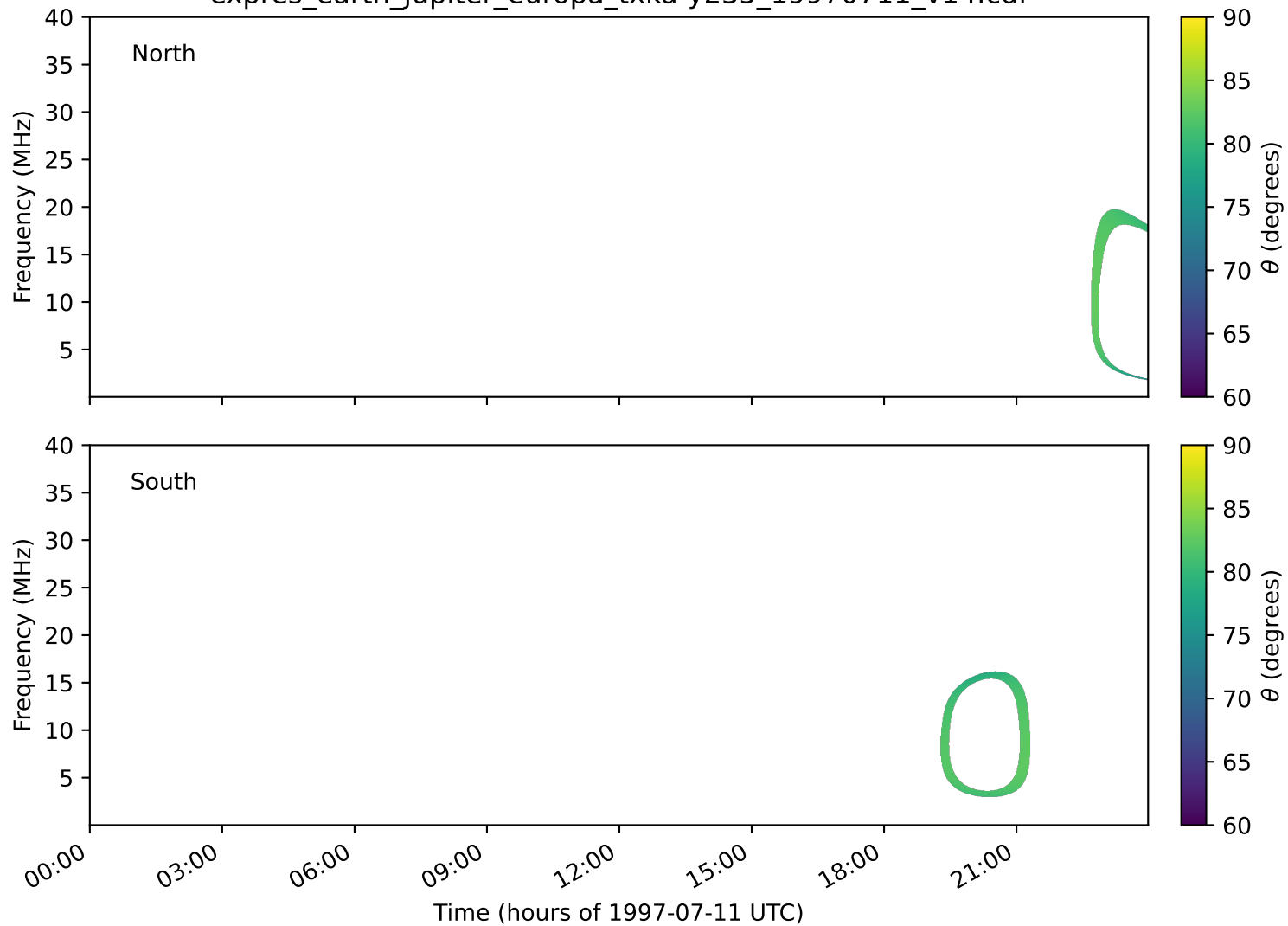
expres_earth_jupiter_europa_txka-y235_19970711_v14.cdf
