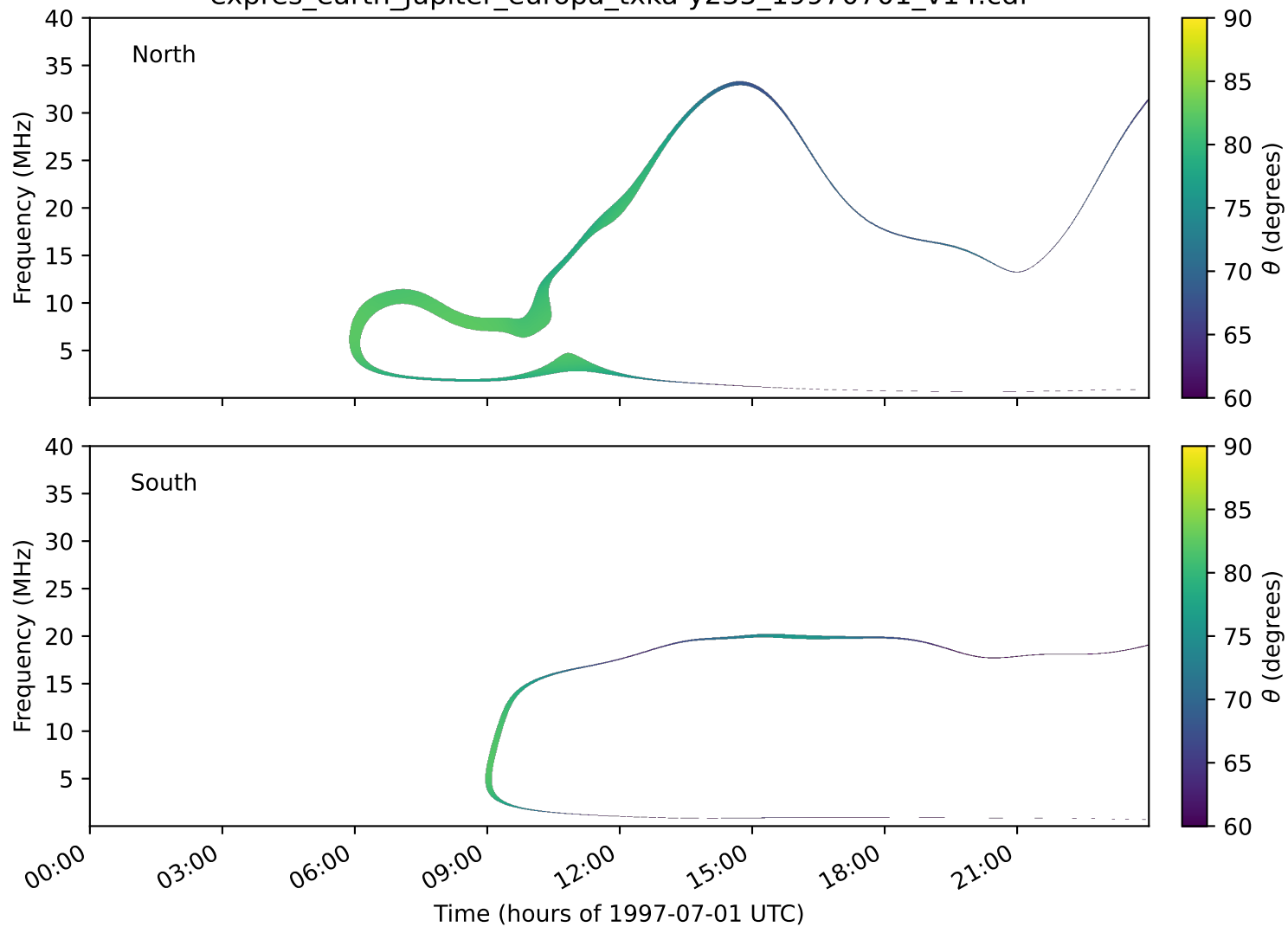
expres_earth_jupiter_europa_txka-y235_19970701_v14.cdf
