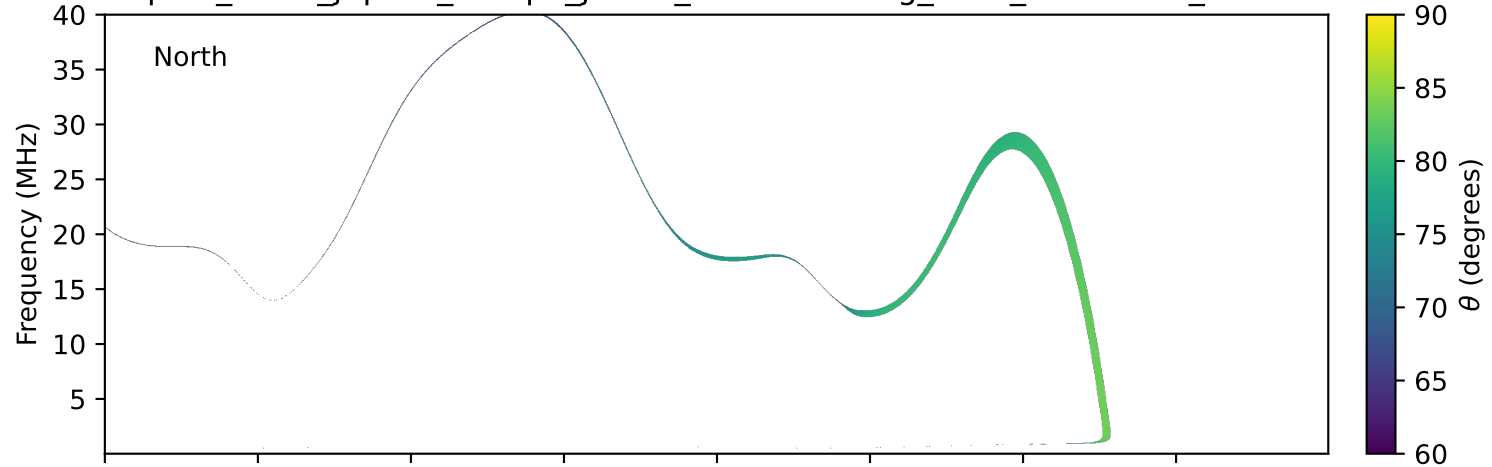
expres_earth_jupiter_europa_jrm33_lossc-wid1deg_3kev_19970727_v11.cdf
