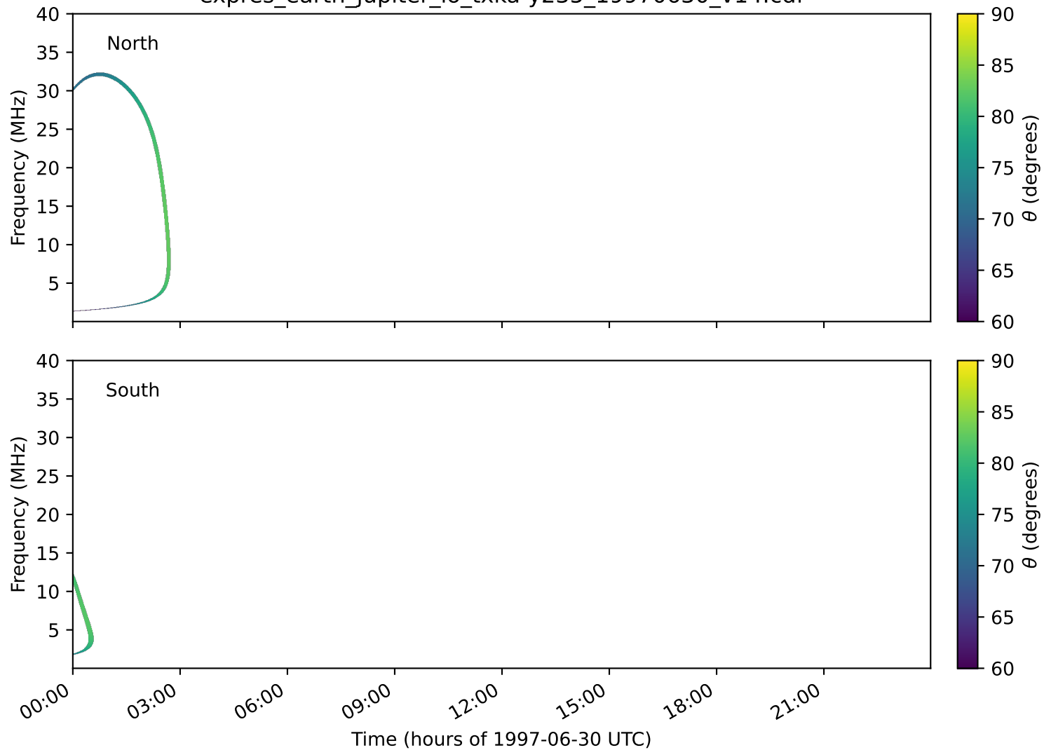
expres_earth_jupiter_io_txka-y235_19970630_v14.cdf
