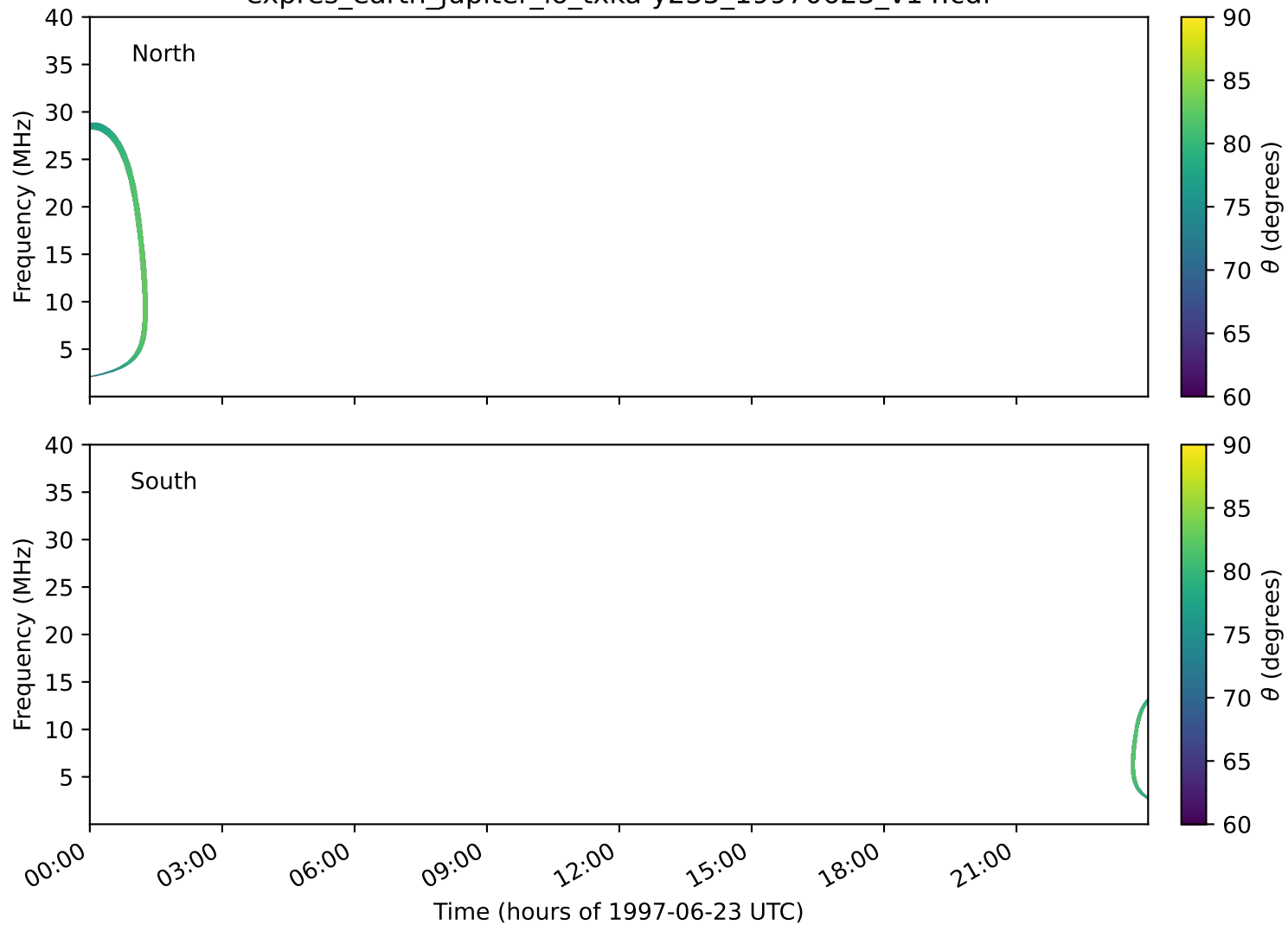
expres_earth_jupiter_io_txka-y235_19970623_v14.cdf
