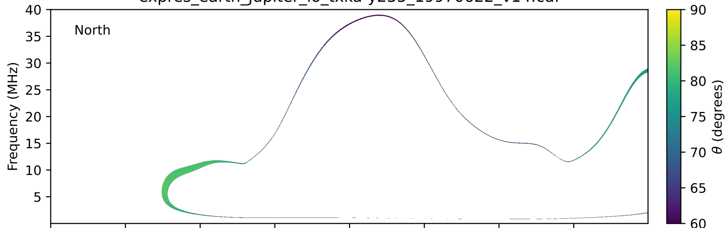
expres_earth_jupiter_io_txka-y235_19970622_v14.cdf
