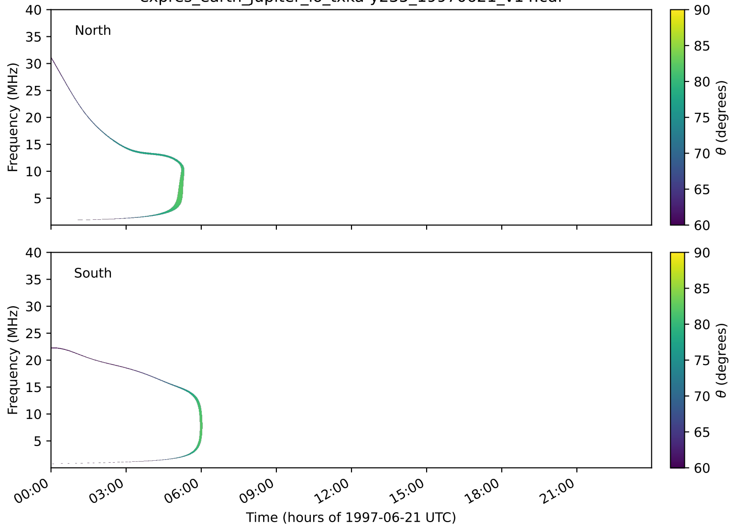
expres_earth_jupiter_io_txka-y235_19970621_v14.cdf
