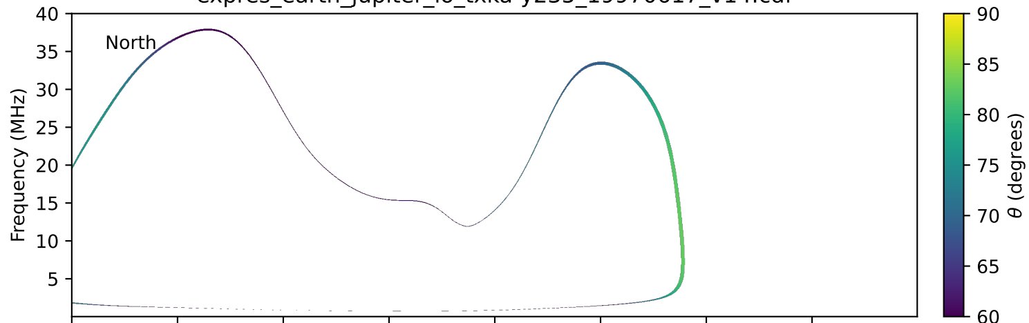
expres_earth_jupiter_io_txka-y235_19970617_v14.cdf
