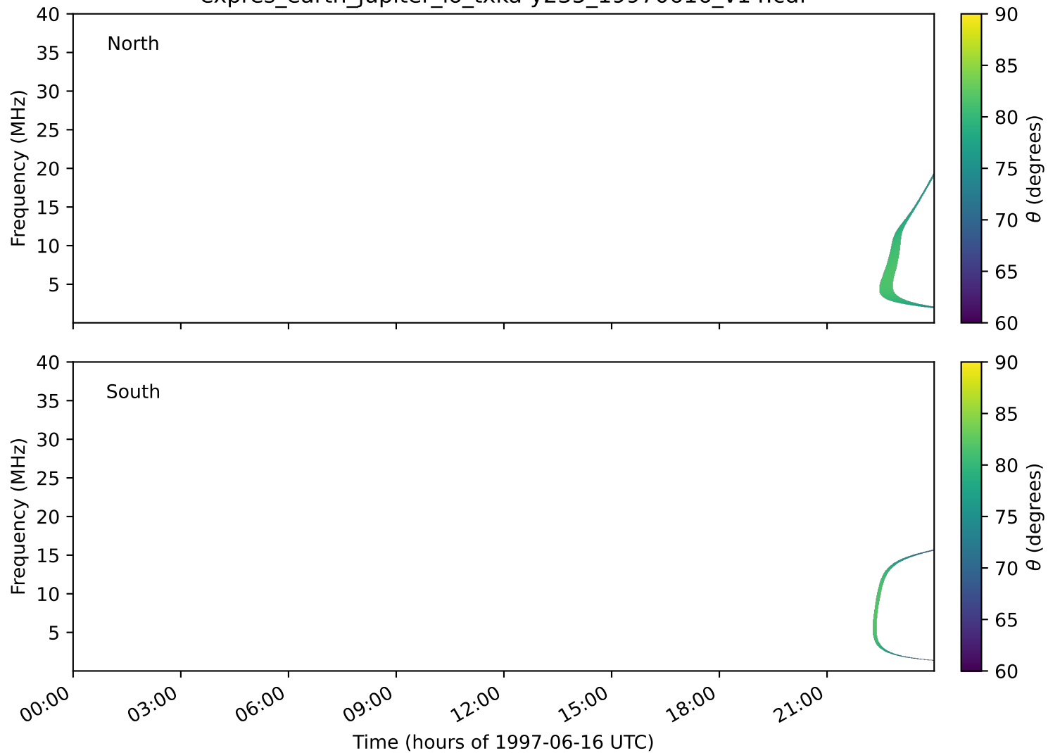
expres_earth_jupiter_io_txka-y235_19970616_v14.cdf
