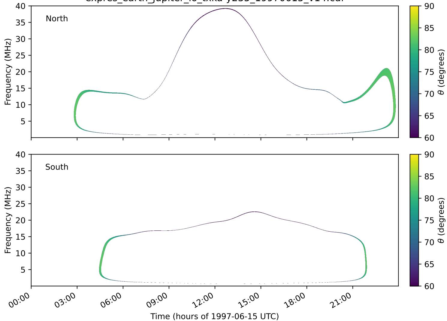
expres_earth_jupiter_io_txka-y235_19970615_v14.cdf
