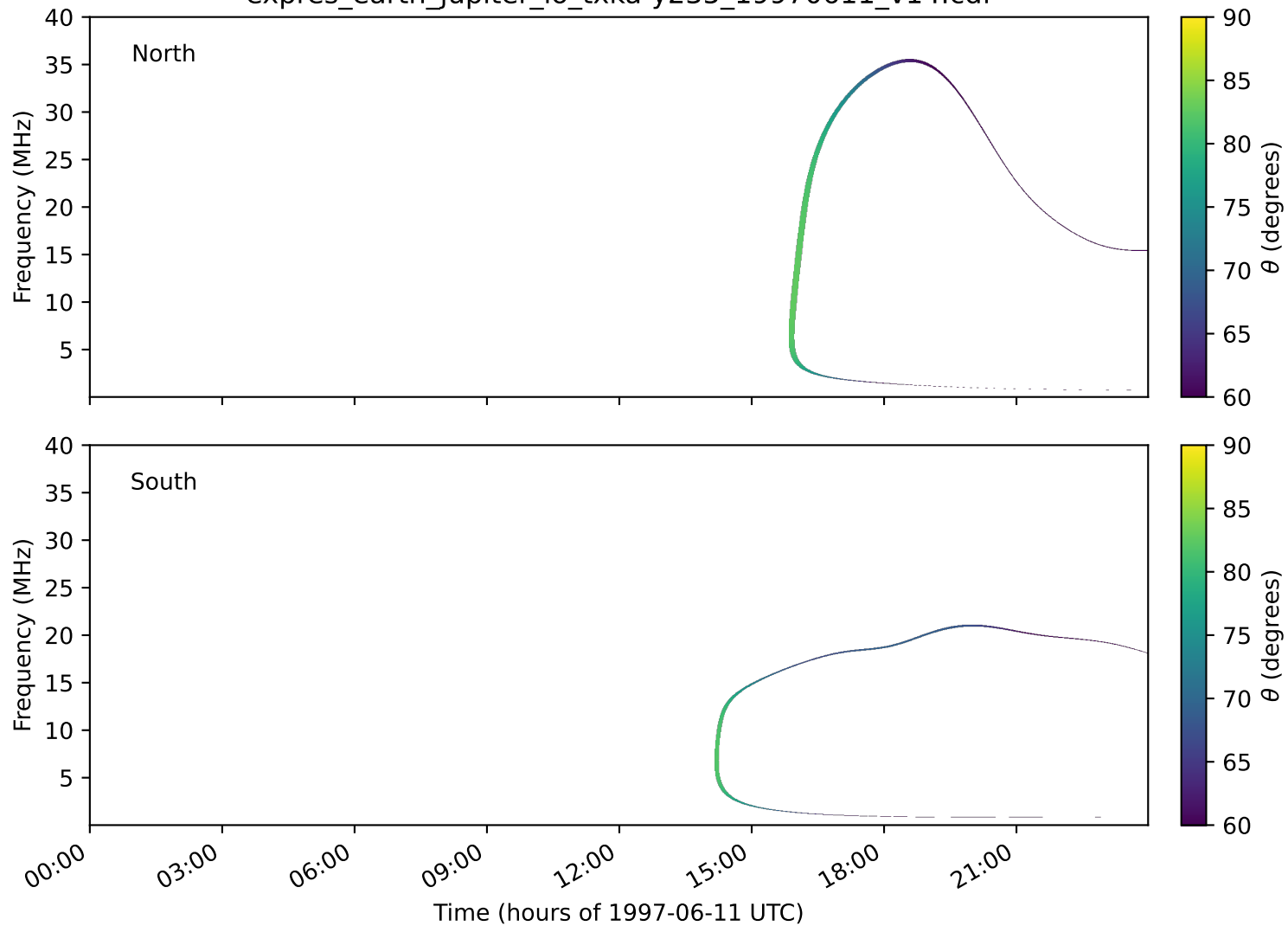
expres_earth_jupiter_io_txka-y235_19970611_v14.cdf
