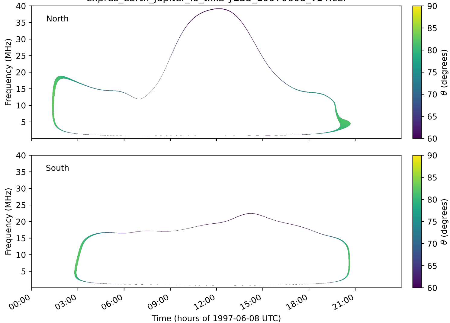
expres_earth_jupiter_io_txka-y235_19970608_v14.cdf
