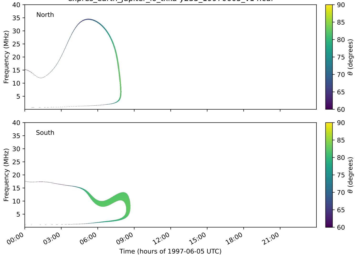
expres_earth_jupiter_io_txka-y235_19970605_v14.cdf
