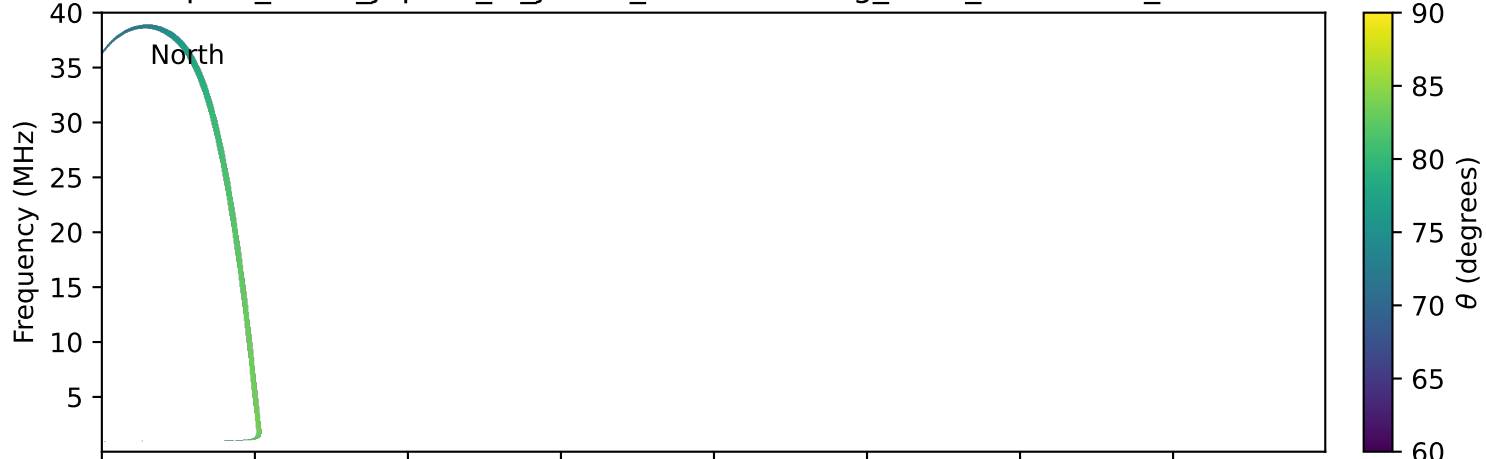
expres_earth_jupiter_io_jrm33_lossc-wid1deg_3kev_19970630_v11.cdf
