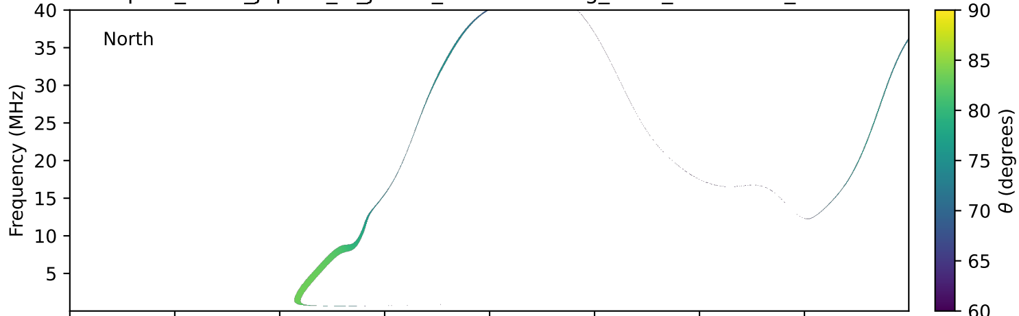
expres_earth_jupiter_io_jrm33_lossc-wid1deg_3kev_19970629_v11.cdf
