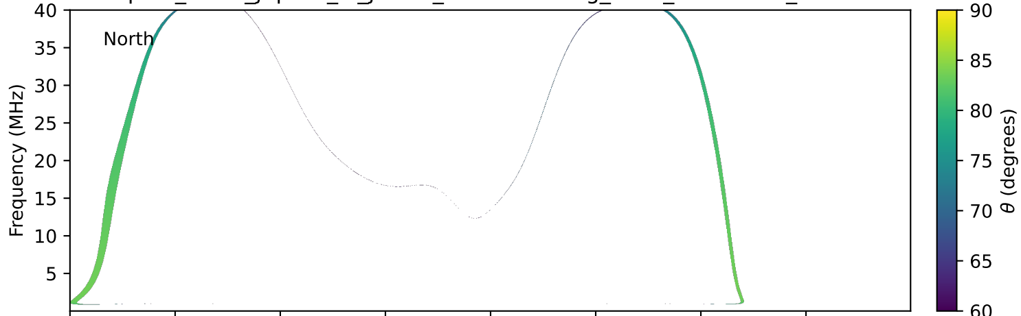
expres_earth_jupiter_io_jrm33_lossc-wid1deg_3kev_19970624_v11.cdf
