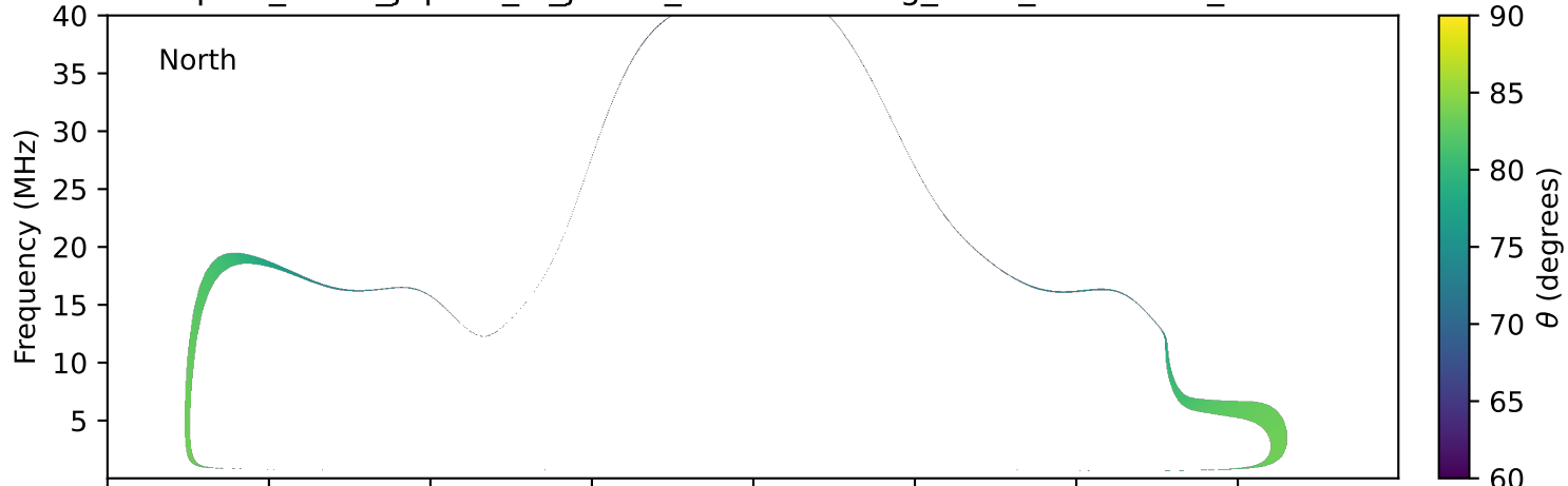
expres_earth_jupiter_io_jrm33_lossc-wid1deg_3kev_19970608_v11.cdf
