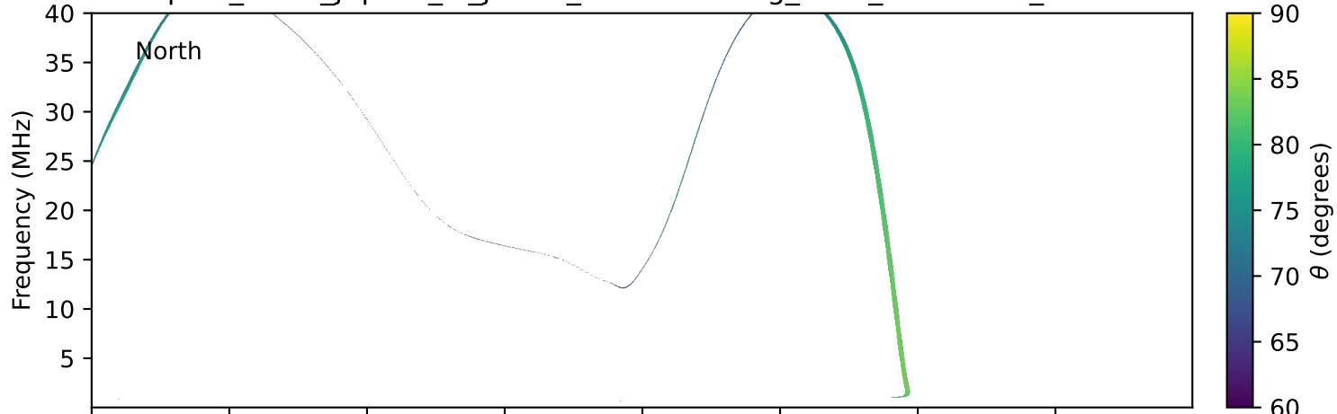
expres_earth_jupiter_io_jrm09_lossc-wid1deg_3kev_19970617_v11.cdf
