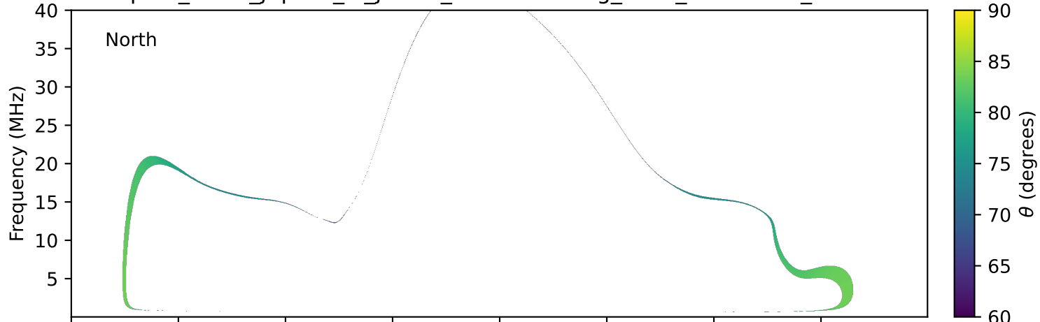
expres_earth_jupiter_io_jrm09_lossc-wid1deg_3kev_19970608_v11.cdf
