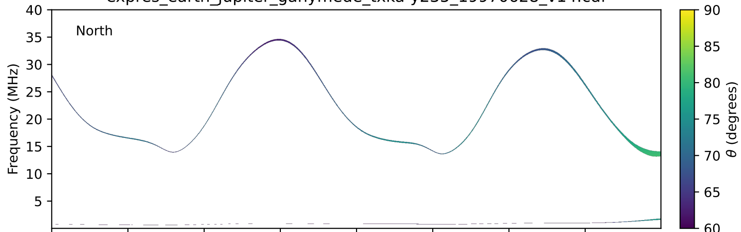
expres_earth_jupiter_ganymede_txka-y235_19970628_v14.cdf
