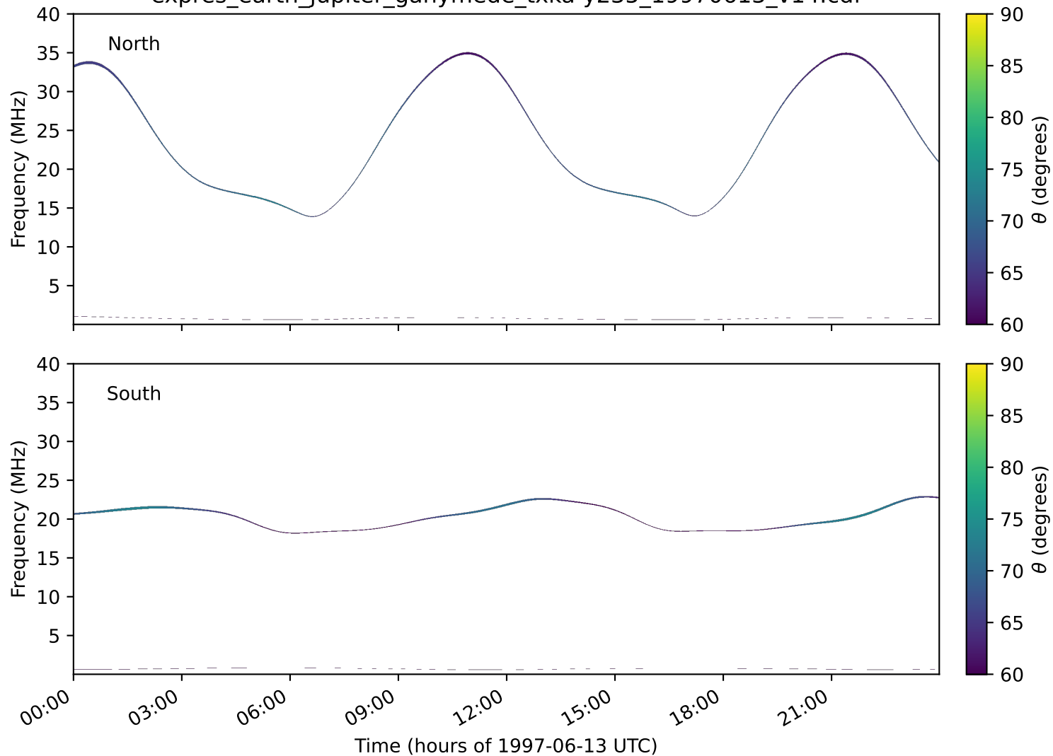
expres_earth_jupiter_ganymede_txka-y235_19970613_v14.cdf
