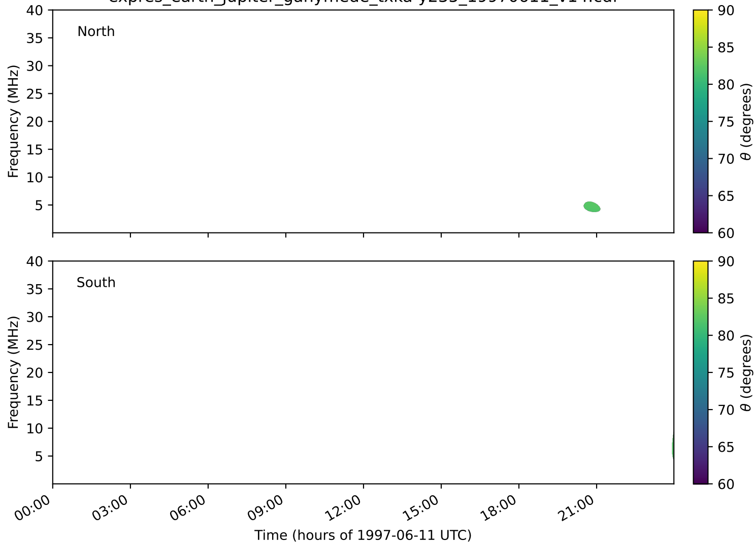
expres_earth_jupiter_ganymede_txka-y235_19970611_v14.cdf
